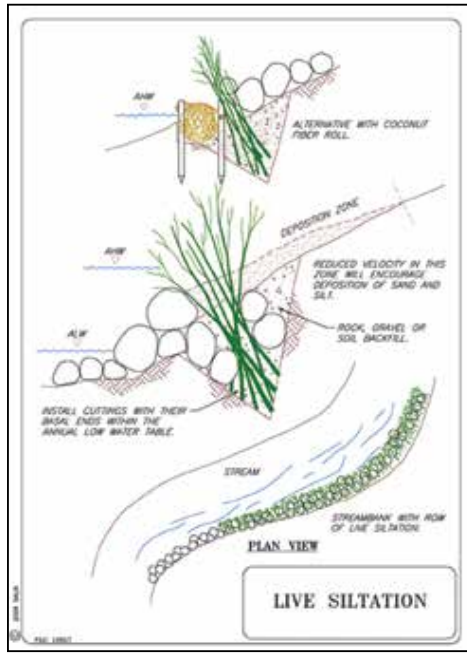
Live Siltation from NCHRP Report 544.
